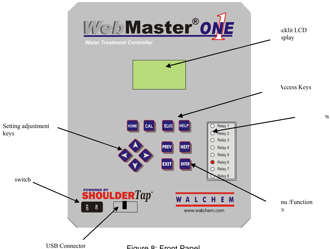
Figure 8: Front Panel
