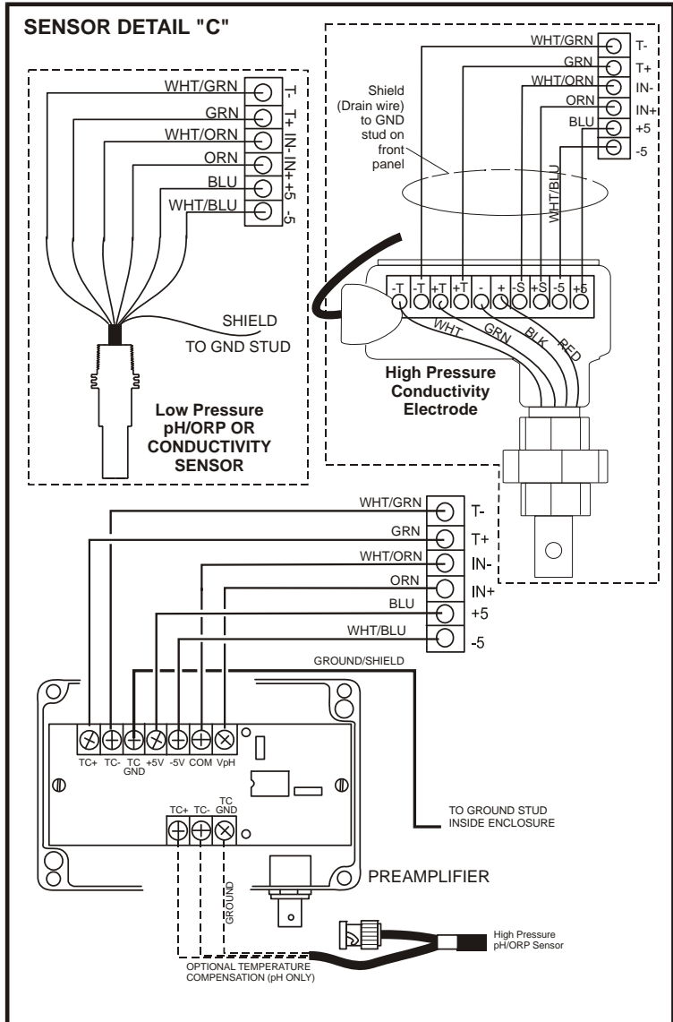
Figure 5: Wiring Diagram for Sensor Inputs and Digital Inputs A-F
