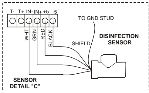
Figure 5: Wiring Diagram for Sensor Inputs and Digital Inputs A-F
